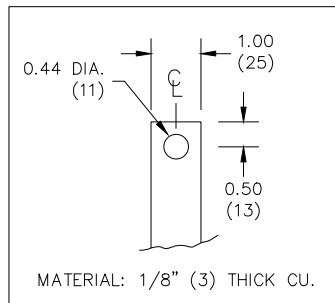
LV TERMINAL DETAIL
