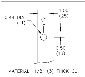
HV TERMINAL DETAIL
