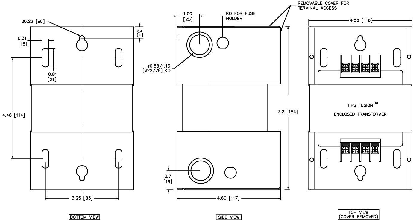
BOTTOM VIEW
