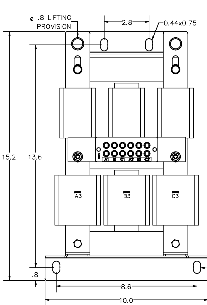
FRONT VIEW
